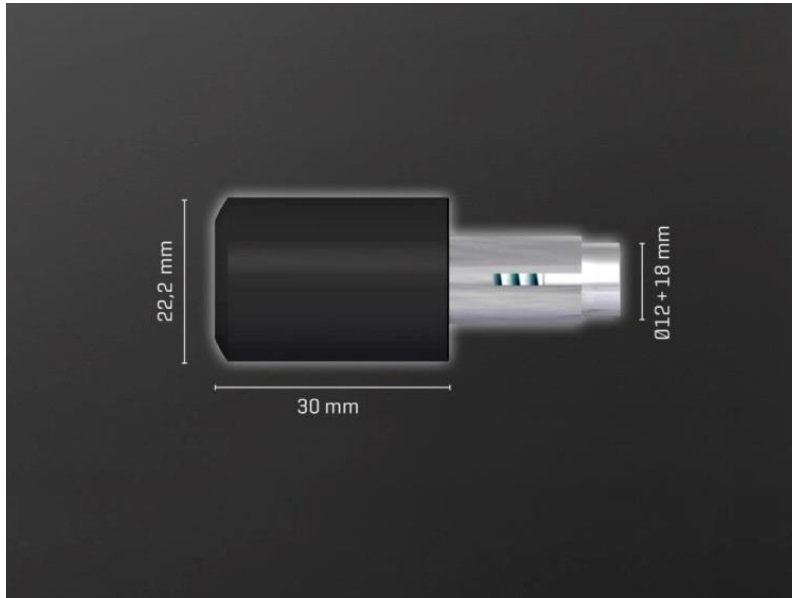
Picture 4 of 4: Two fastening sleeves are included (for inner diameters 12 & 18 mm)
